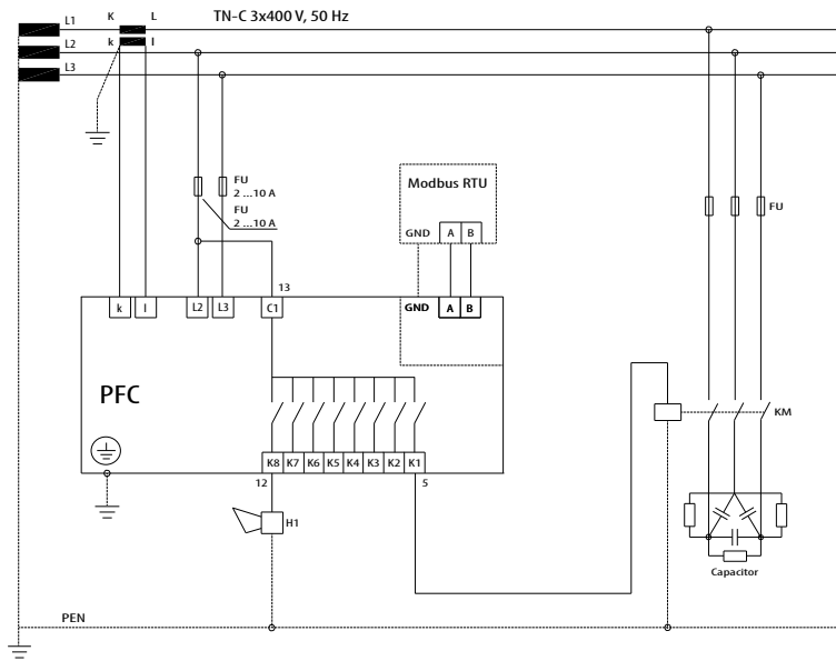
PFC 8 electrical scheme
