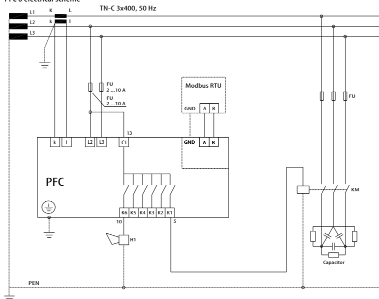
PFC 6 electrical scheme
