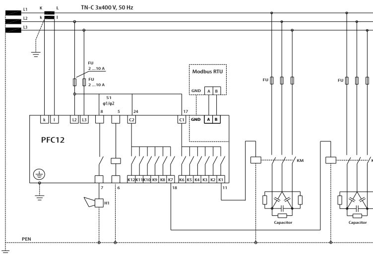
PFC 12 electrical scheme
